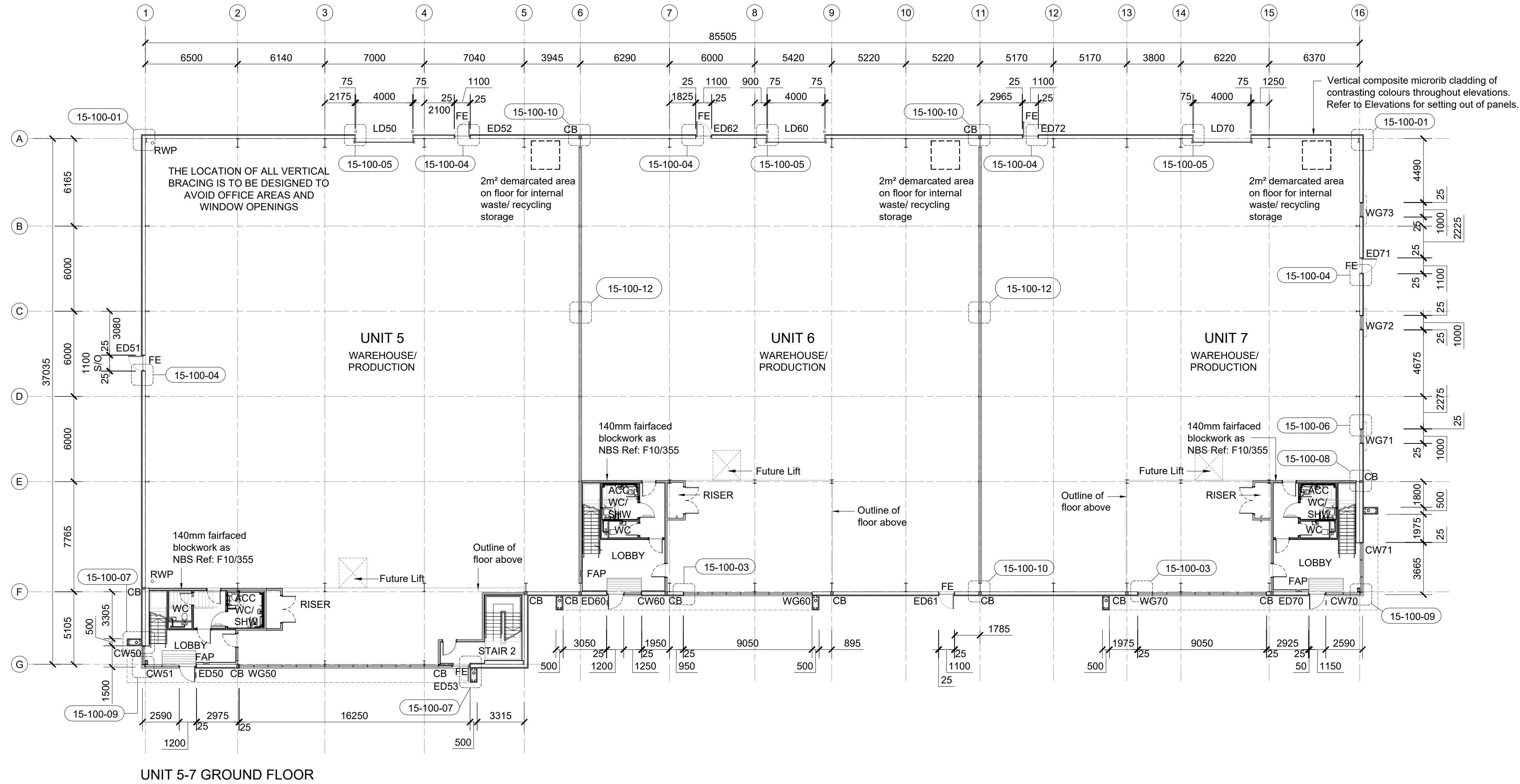
UNIT 5-7 GROUND FLOOR
